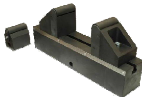
600 kN Flexure Fixture
